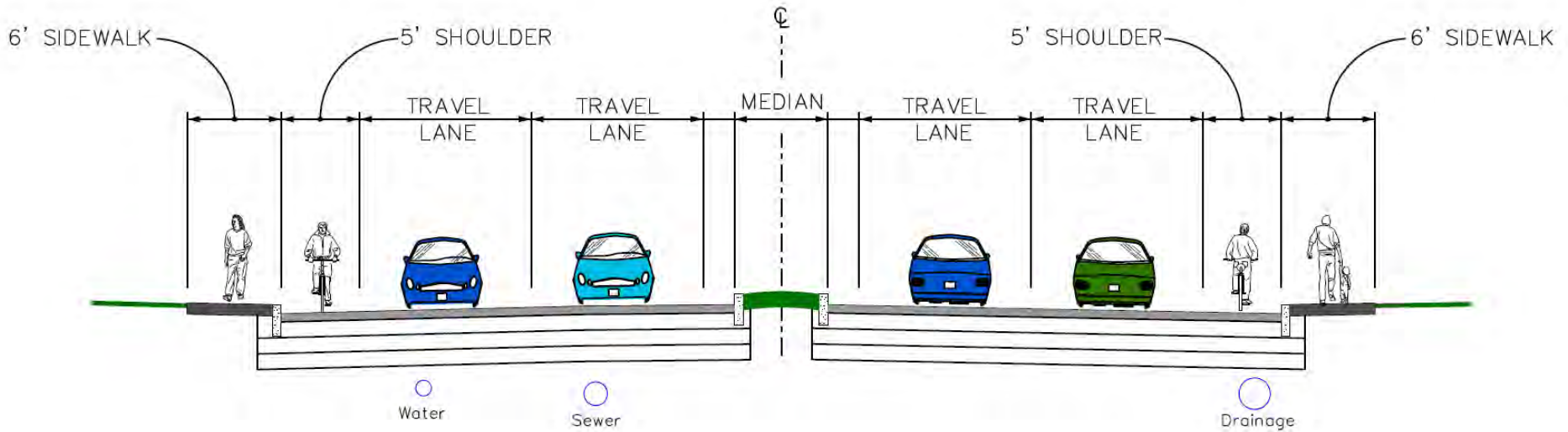
WINCHESTER STREET - TYPICAL SECTION
